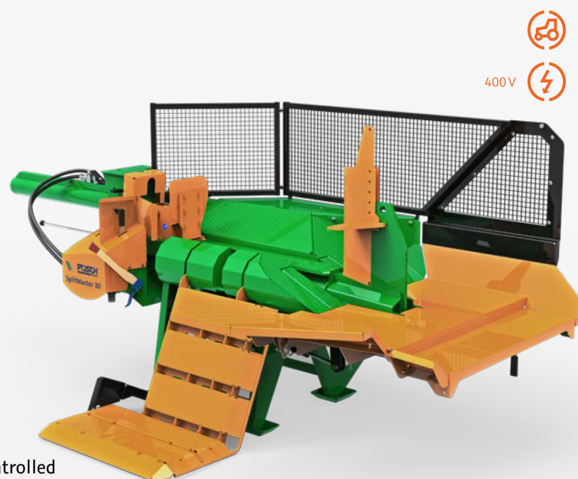
SplitMaster 30 with 4-blade knife in working position
